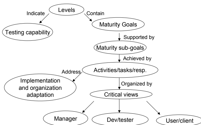
Fig 1: The internal structure of TMM maturity levels Courtesy: Practical Software Testing by Ilene Burnstein
